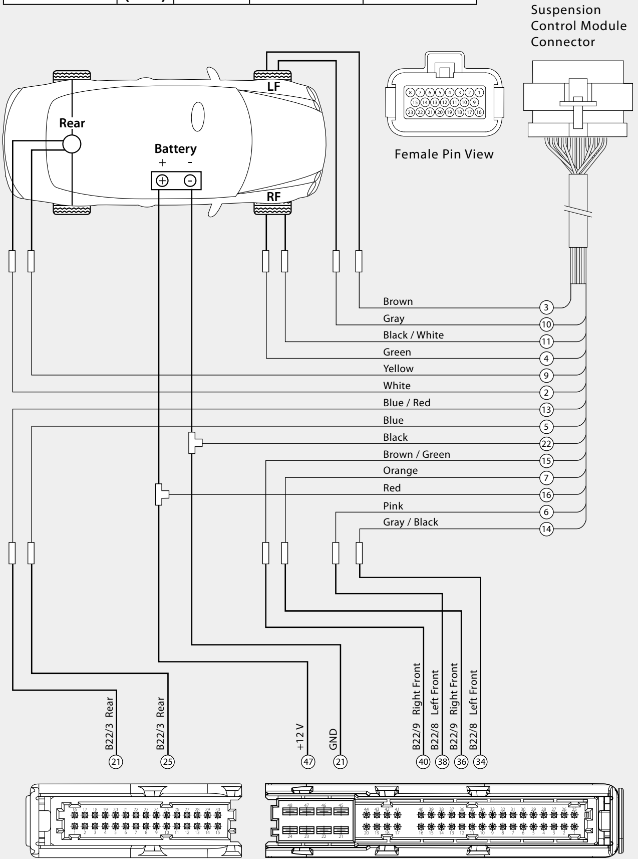
Airmatic Harness, Female Pin View
