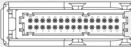
Airmatic Harness, Female Pin View
